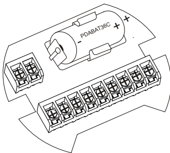
Figure 14. Battery Orientation
