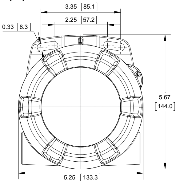
Figure 16. Enclosure Dimensions – Front View
