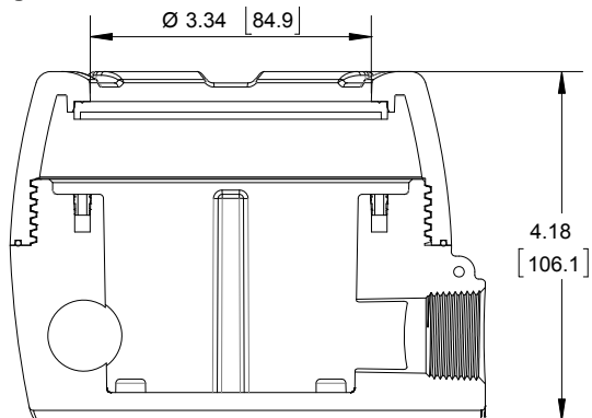
Figure 17. Enclosure Dimensions – Side Cross Section View
