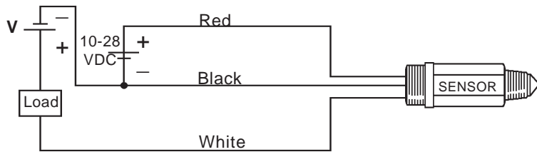
Figure 2 External Load
